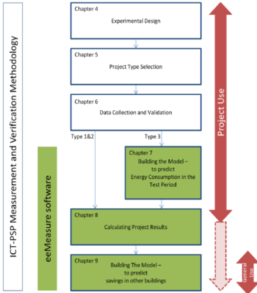
Figure 2: ICT-PSP measurement and verification methodology flowchart - (eeMeasure) – D1.2 Non-residential methodology
