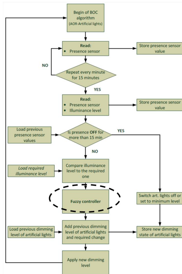
Figure 1: Lighting algorithm structure
